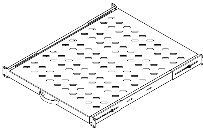
ISOMETRIA
