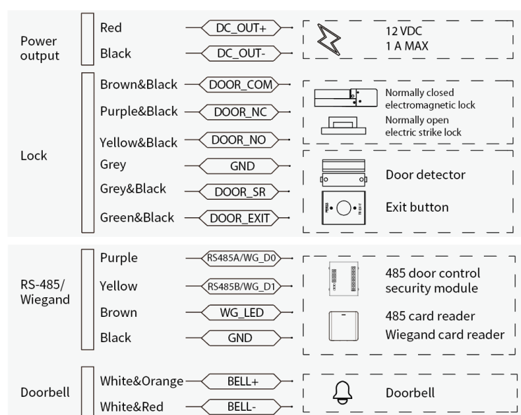
Figure 2-5 Wiring
