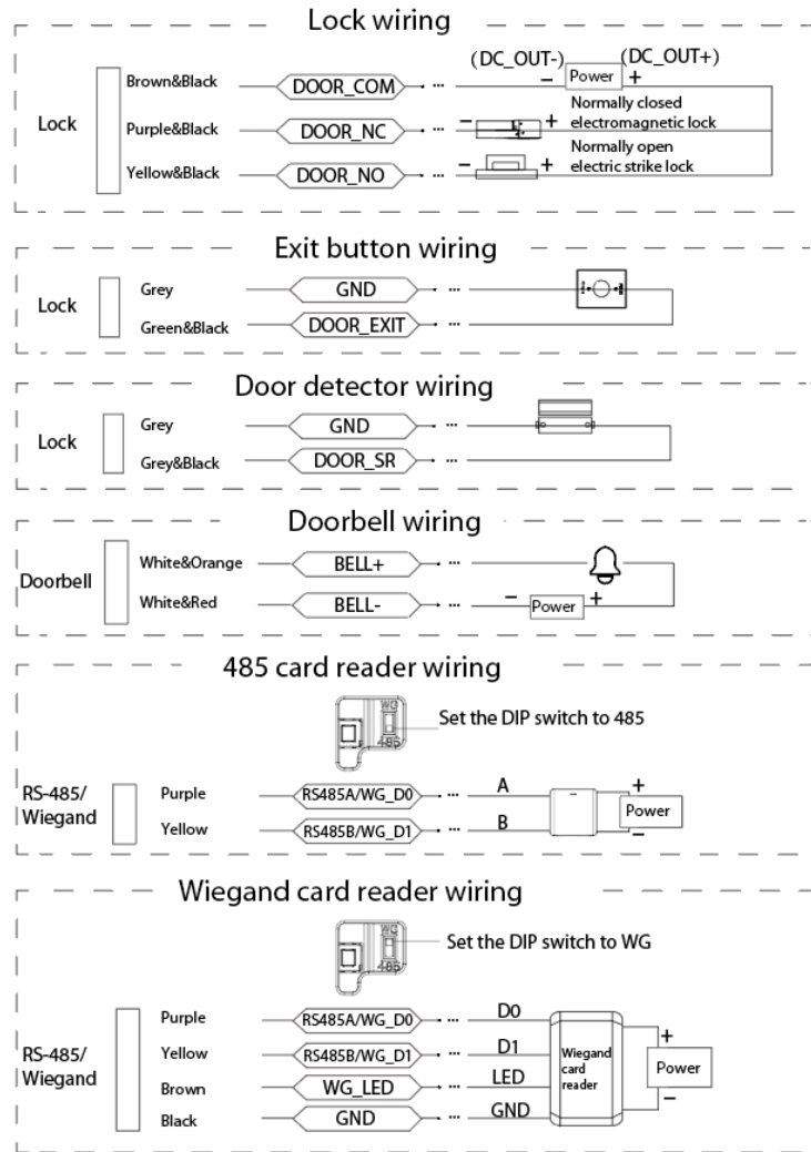
Figure 2-7 Wiring for the door control security module
