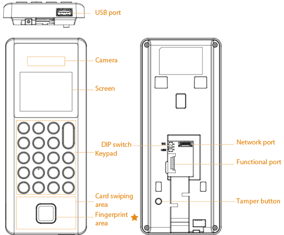
Figure 1-1 Structure
