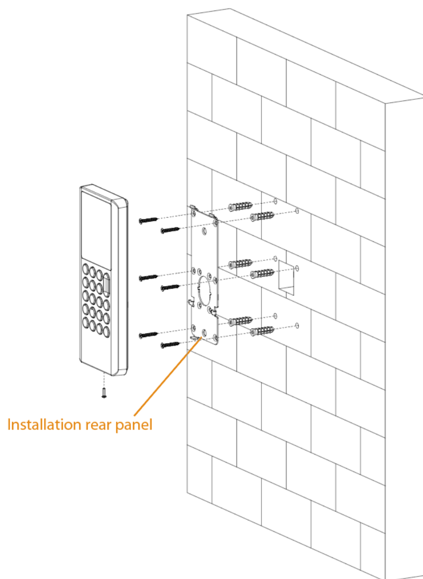
Figure 2-8 In-wall wiring
