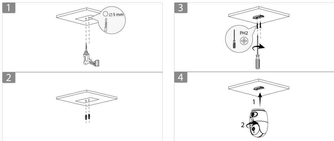
Figure 3-5 Ceiling mount
